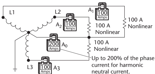
9-6 Effect of harmonics due to nonlinear loads.
